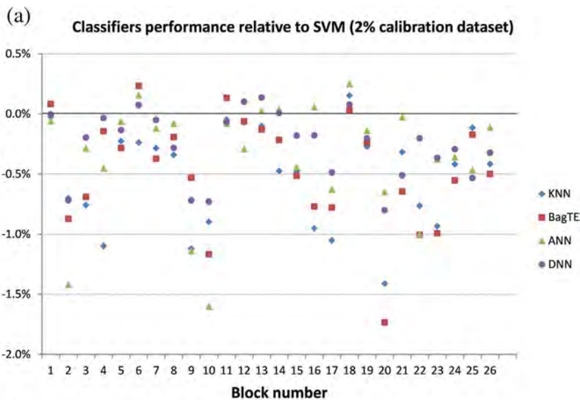
Fig. 2. Classifiers overall accuracy relative to SVM for (a) 2% and (b) 0.2% calibration dataset.
