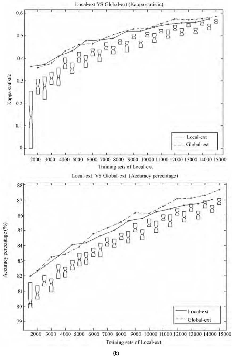
Figure 5. Comparison between Local and Global models using decision tree algorithms. (a) Decision trees assessment within the interior subregion; (b) Decision trees assessment within the exterior subregion.
